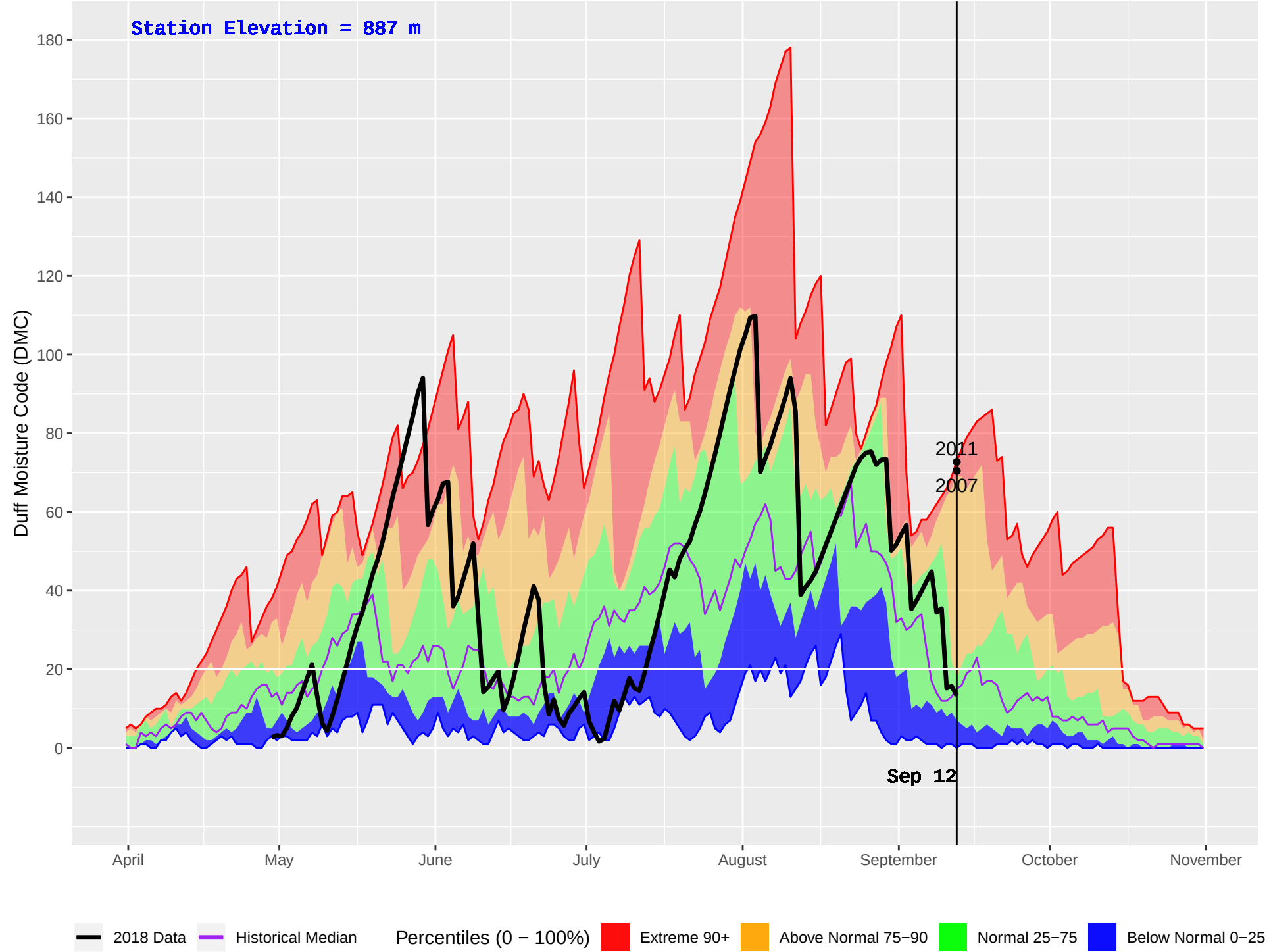
CRAWFORD (873) : Historical (2004–2016) and Current (2018) Daily Duff Moisture Code (DMC)
