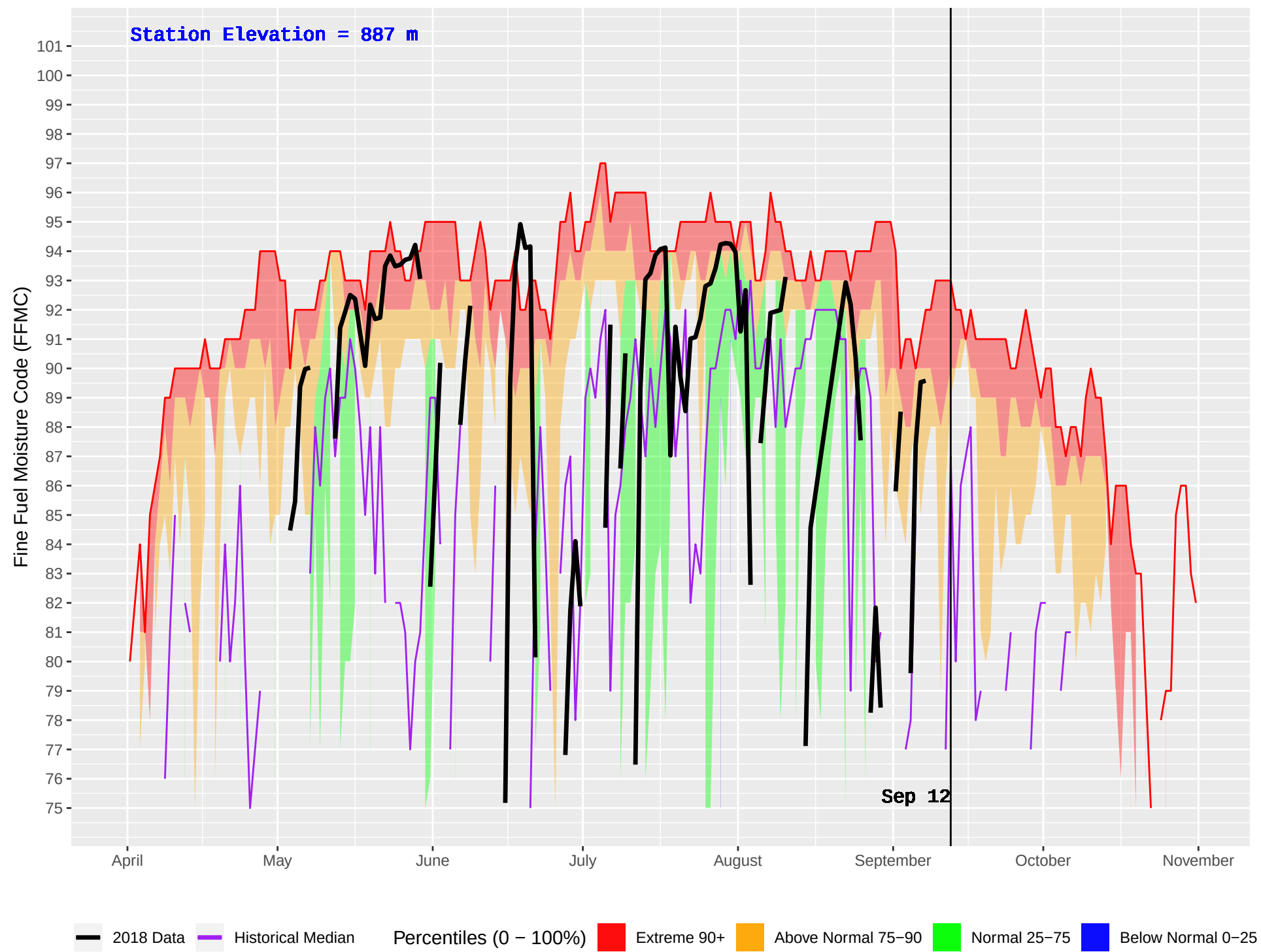
CRAWFORD (873) : Historical (2004–2016) and Current (2018) Daily Fine Fuel Moisture Code (FFMC)
