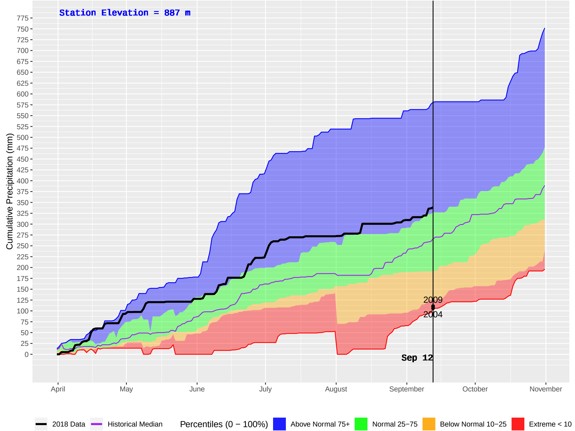
CRAWFORD (873) : Historical (2004–2016) and Current (2018) Daily Cumulative Precipitation
