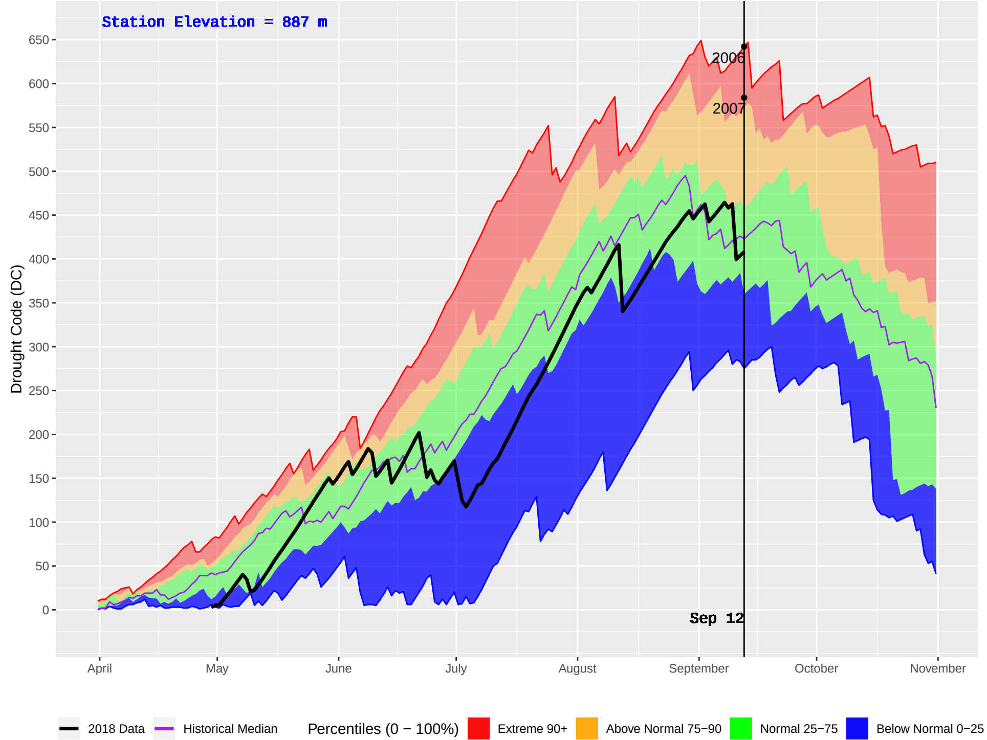
CRAWFORD (873) : Historical (2004–2016) and Current (2018) Daily Drought Code (DC)
