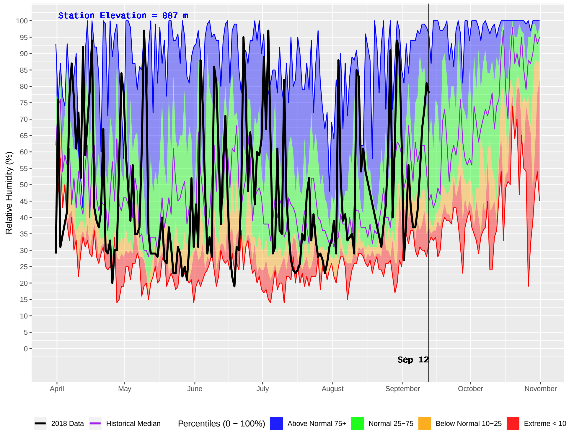
CRAWFORD (873) : Historical (2004–2016) and Current (2018) Daily Relative Humidity
